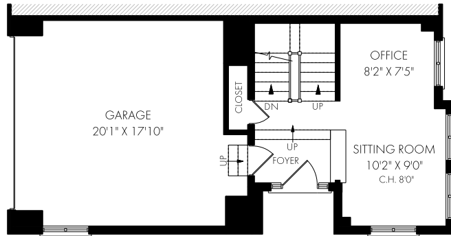
GROUND LEVEL - 336 SQUARE FEET
