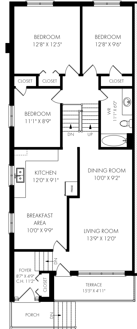
CEILING HEIGHT 8'0" MAIN LEVEL - 651 SQUARE FEET UPPER LEVEL - 615 SQUARE FEET
