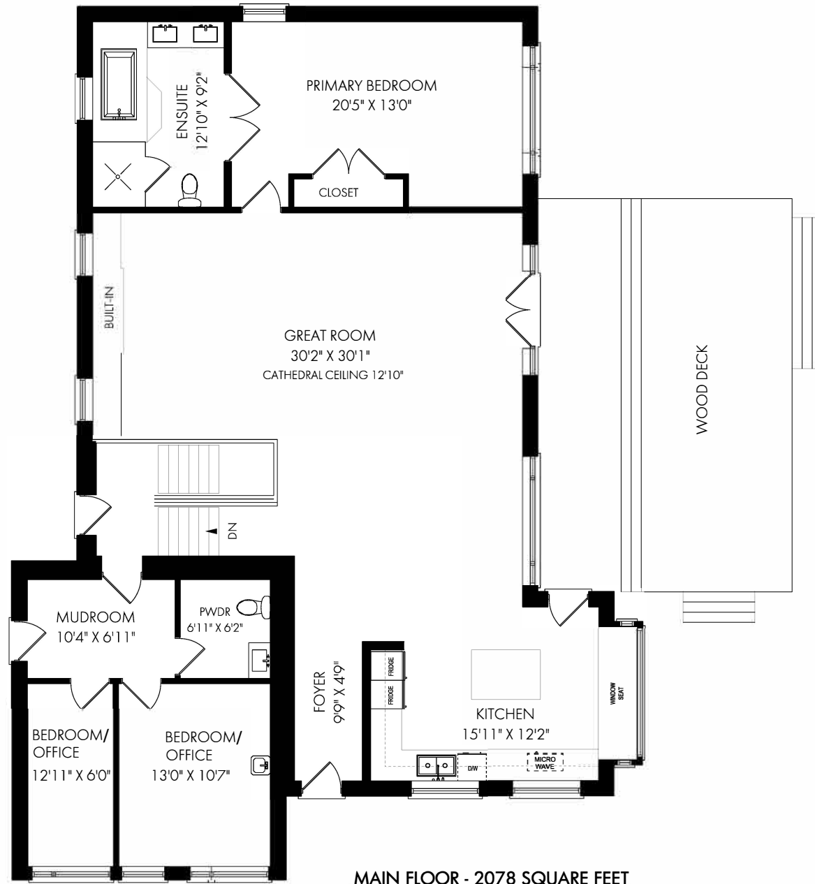
MAIN FLOOR - 2078 SQUARE FEET
