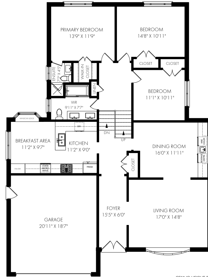
CEILING HEIGHT 8'0" MAIN LEVEL - 943 SQUARE FEET UPPER LEVEL - 779 SQUARE FEET
