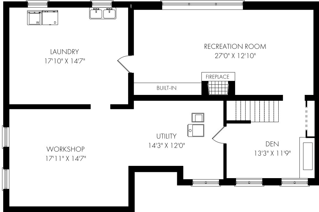
LOWER LEVEL - 1385 SQUARE FEET
