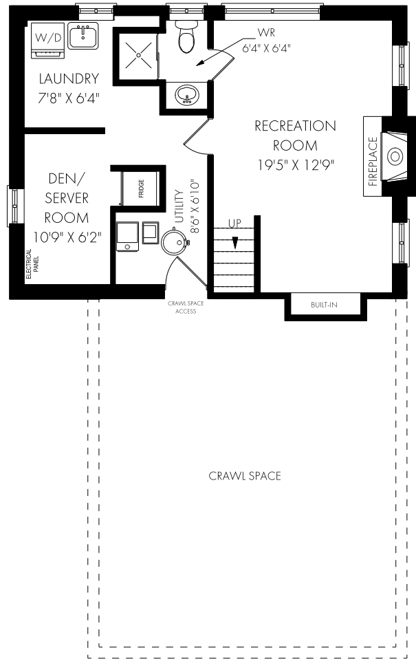
LOWER LEVEL - 601 SQUARE FEET
