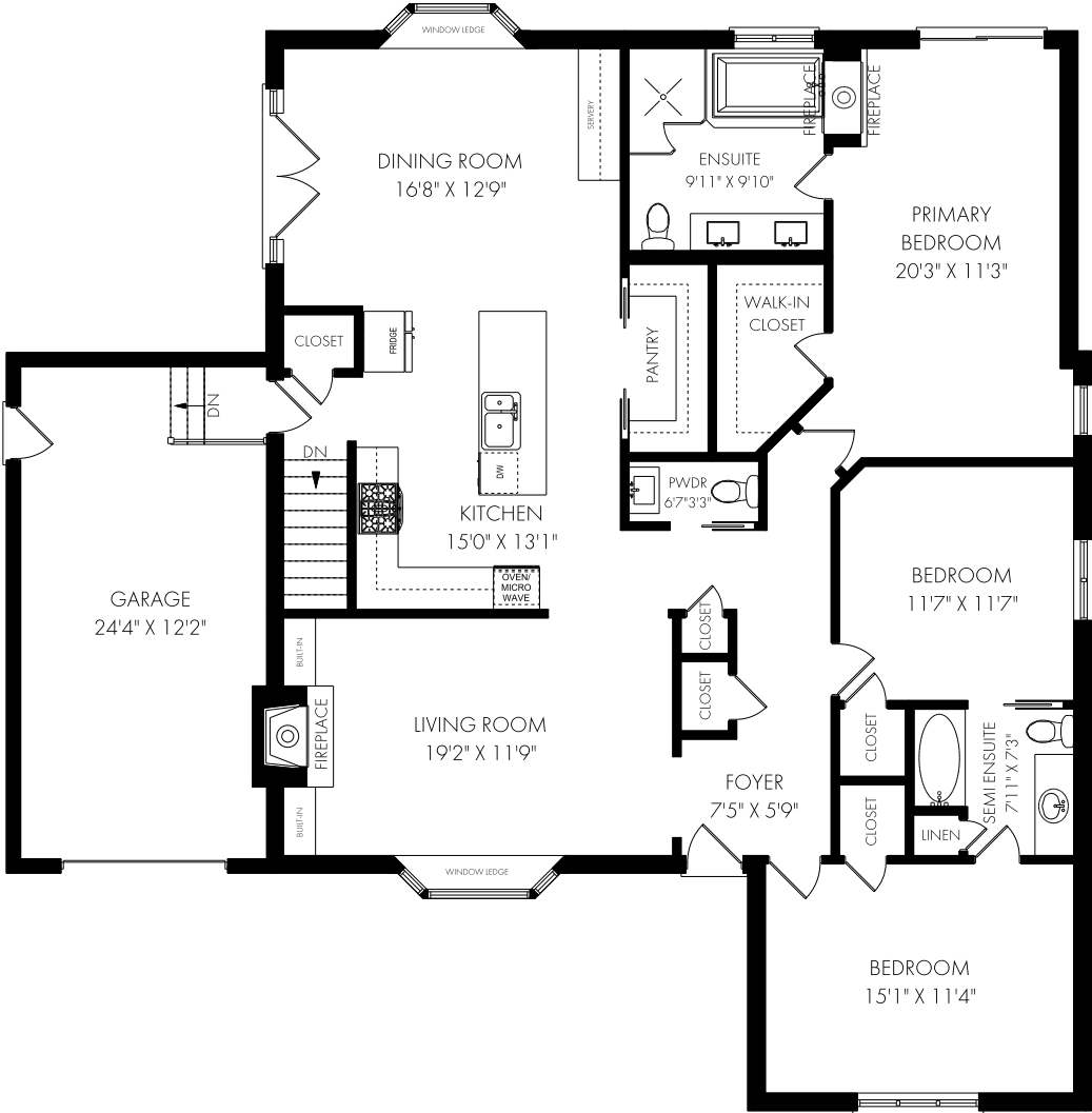
CEILING HEIGHT 8'0" MAIN FLOOR - 1907 SQUARE FEET
