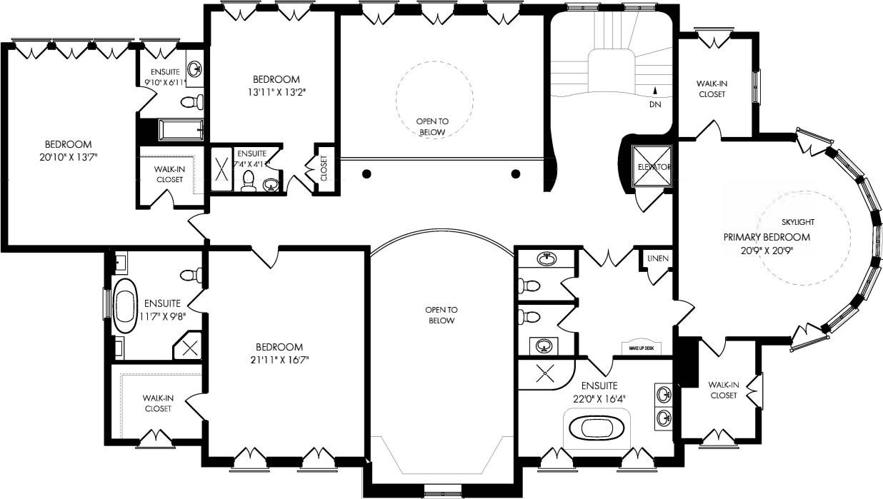
CEILING HEIGHT 9'10" SECOND FLOOR - 3147 SQUARE FEET AREA EXCLUDES 685 SQ.FT. OPEN TO BELOW SPACE
