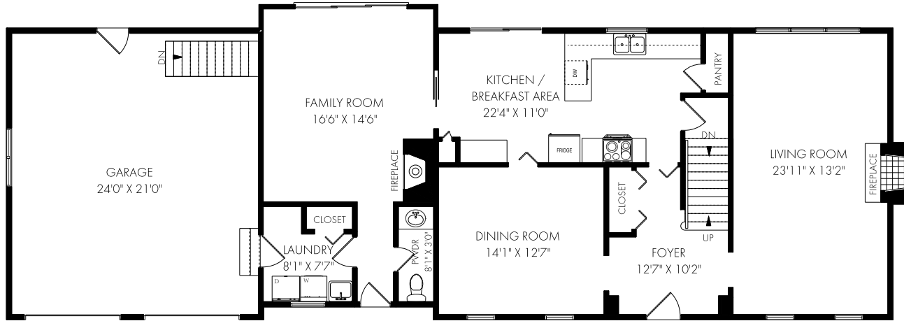
MAIN FLOOR - 1356 SQUARE FEET
