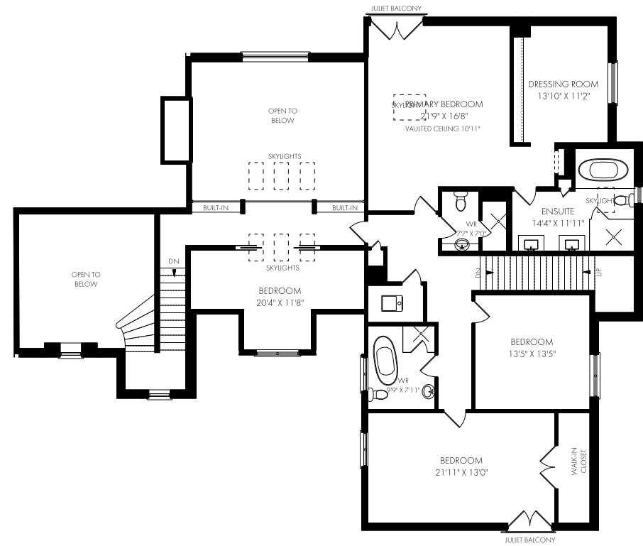
SECOND FLOOR - 2193 SQUARE FEET
