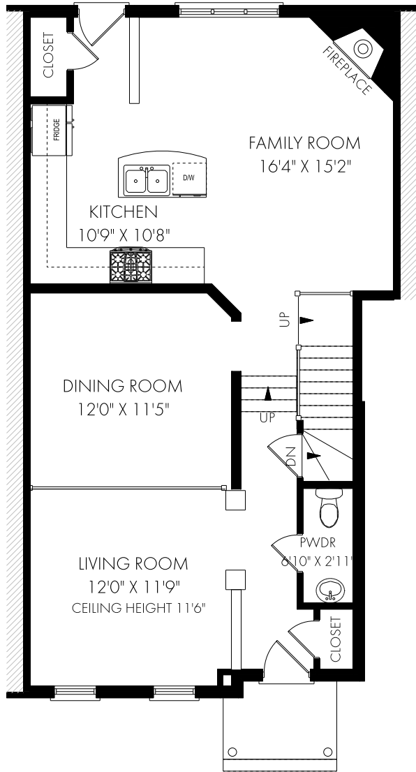
CEILING HEIGHT 9'0" MAIN FLOOR - 872 SQUARE FEET
