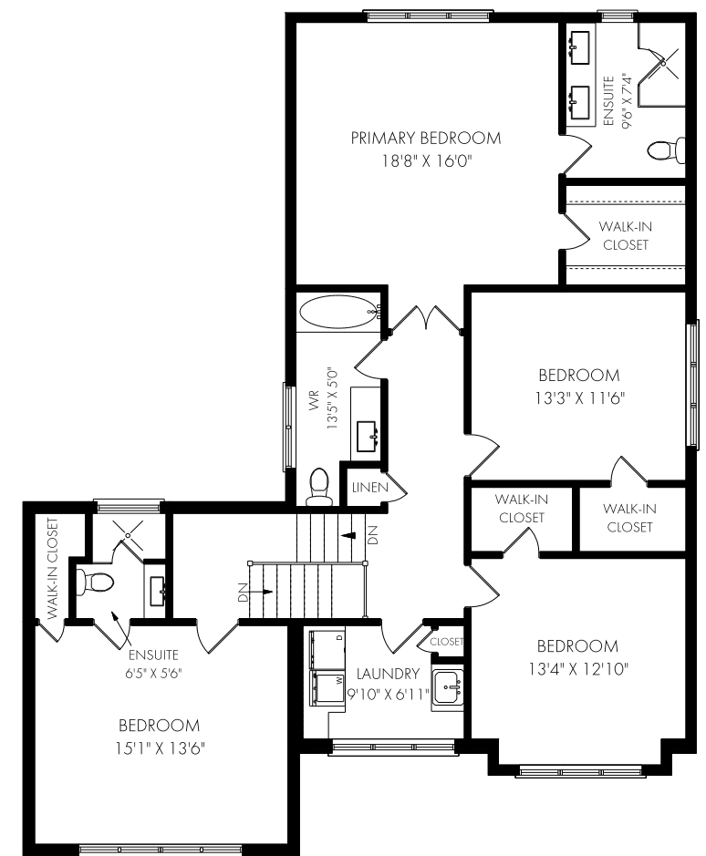
CEILING HEIGHT 8'0" SECOND FLOOR - 1493 SQUARE FEET
