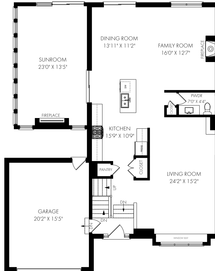
CEILING HEIGHT 8'10" MAIN FLOOR - 1510 SQUARE FEET
