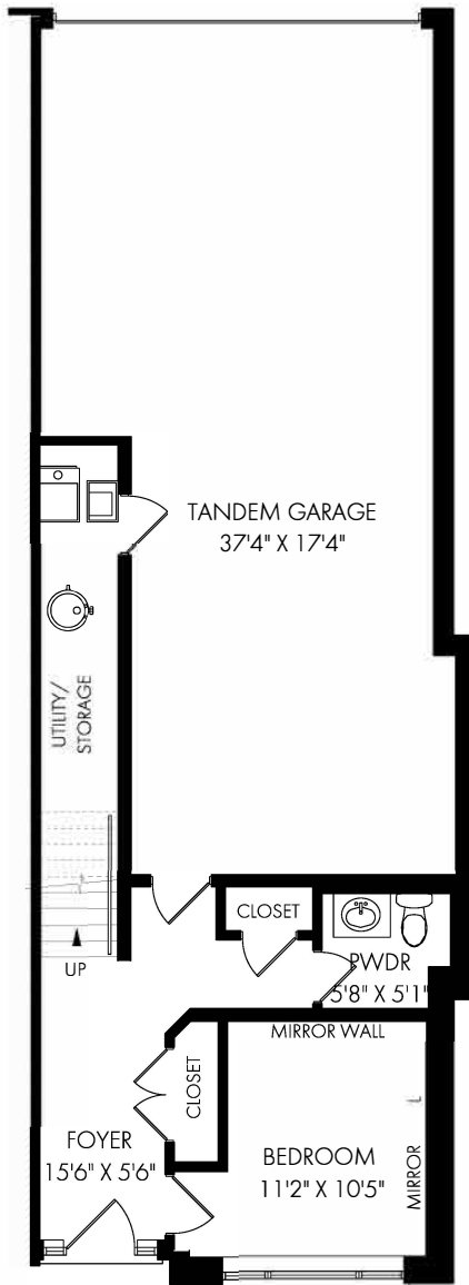
GROUND FLOOR - 334 SQUARE FEET
